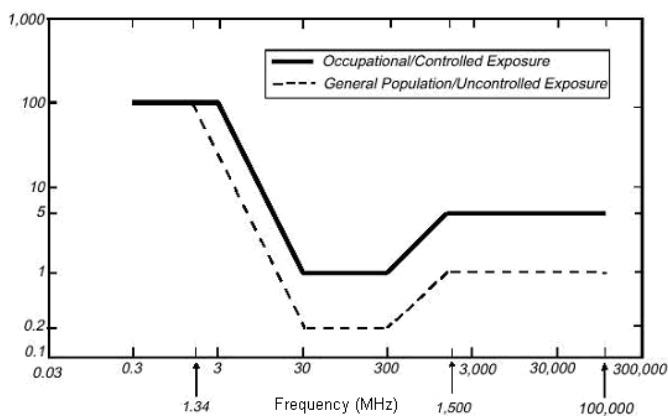
FCC MPE (power density, \text{mW/cm}^2 , vs MHz): solid occupational, dashed public.
